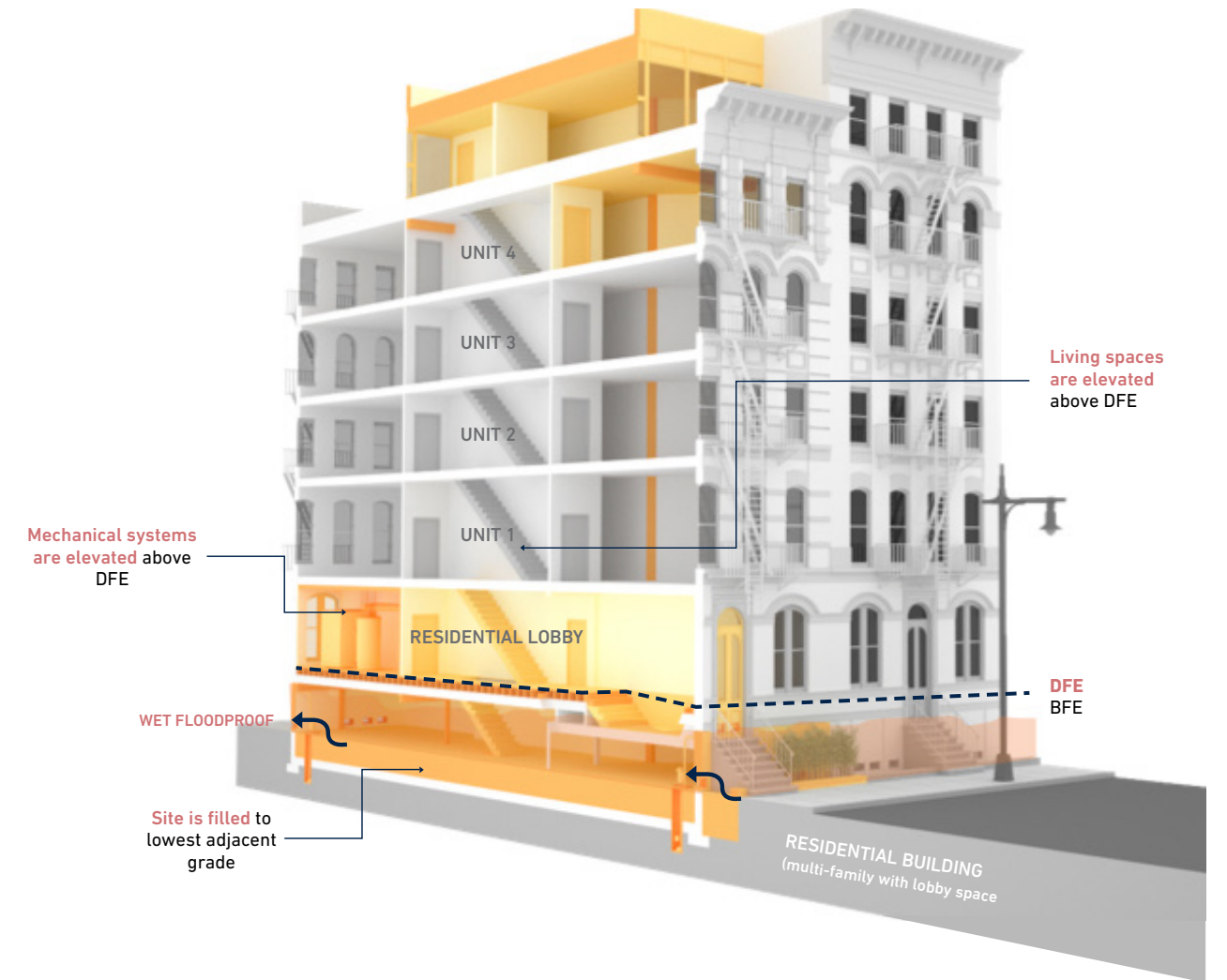
EXAMPLES OF RETROFITTING BUILDINGS FOR FLOOD RISK SOURCE: NYC DCP
