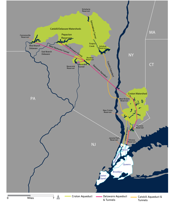
NEW YORK CITY'S WATER SUPPLY SYSTEM SOURCE: NYC DEP
